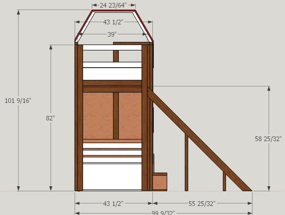
LEFT VIEW
