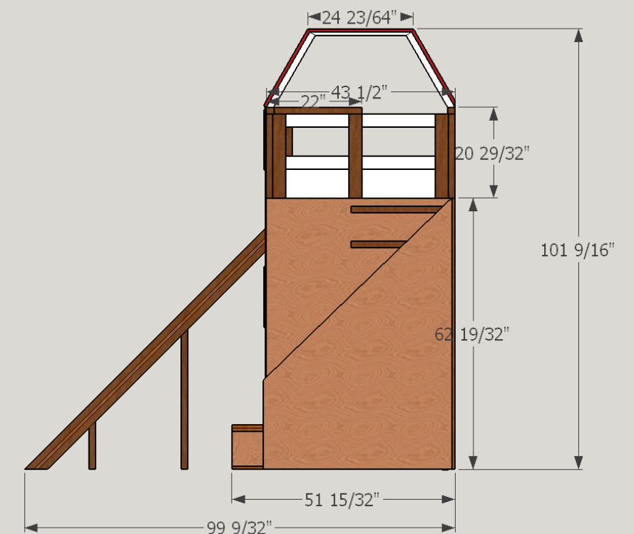
RIGHT VIEW
