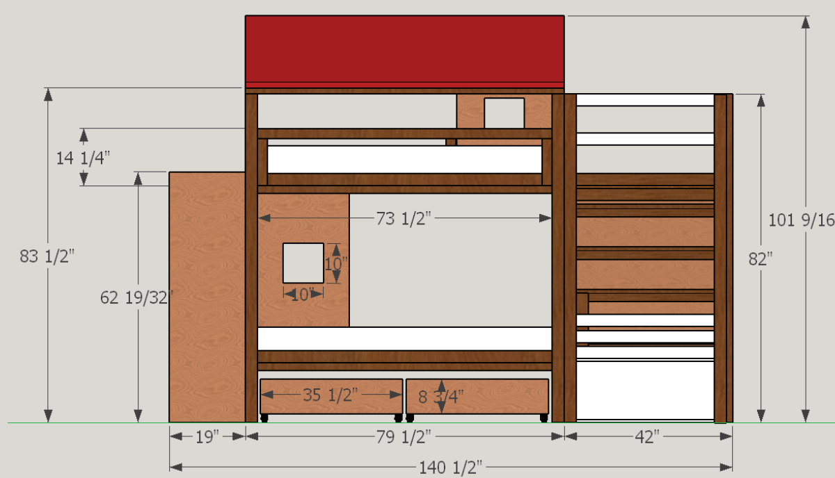
LEFT VIEW
